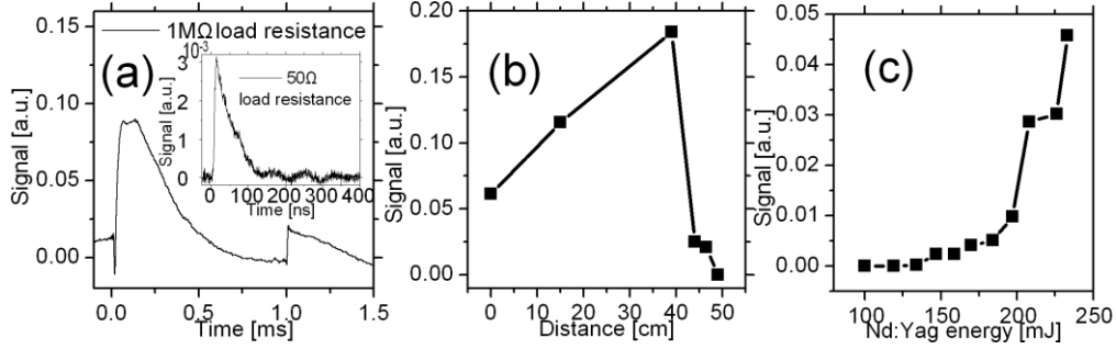
Fig. 2. (a) Signal detected using the electrical method, showing plasma channel initially created by the fs laser and then revived by the ns laser (532 nm) after 1 ms. (b) Magnitude of the signal from the revived plasma at various distances from the beginning of the initial plasma filament. (c) Magnitude of the signal from the revived plasma as a function of the Nd:YAG laser pulse energy. In (b) and (c) each point corresponds to the average of 100 measurements. The mean fluctuation around the average is 5%.
