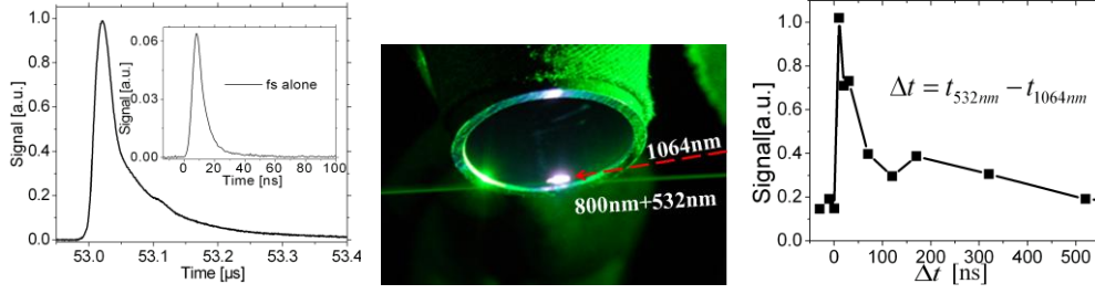
Fig. 3. Three beam configuration when both YAG laser pulses are delayed by 53 \mu s from the fs laser pulse: (a) Signals detected by the PMT with a 338 nm filter in the presence of breakdown. The laser pulse at 1064 nm arrives 10 ns after the pulse at 532 nm. The optical signal recorded under the same conditions with the fs laser alone is shown in the inset (the magnitudes can be compared). (b) Photograph of the breakdown spark in a three laser beams configuration. The beam paths are shown with dotted lines. (c) Revival plasma triggered breakdown probability as a function of delay between the 1064 nm and 532 nm. A positive delay corresponds to the 532 nm pulse arriving first. Each point is an average over 1000 shots.
