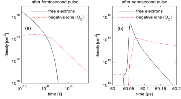
Fig. 4. Evolution of free electron and O_2^- ion densities: (a) After the fs laser excitation. (b) During and after the delayed ns pulse (at 532 nm) excitation. The end of the time axis in (a) coincides with the beginning of time axis in (b). The fs pulse arrives at t = 0 and creates the initial plasma channel of density 10^{17} \text{ cm}^{-3} . The ns pulse is a Gaussian with 10 ns (FWHM) duration, has its peak 50 ns after the beginning of time axis of (b) (at 50.05 \mu\text{s} ) and it has a peak intensity of 10^{11} \text{ W/cm}^2 .
