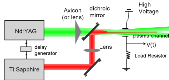
Fig. 1. Experimental setup. The fs laser generates the plasma channel and the delayed ns laser revives it. The plasma channel is detected using electrodes with high voltage and/or a PMT.
