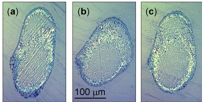
Fig. 5. (a), (b) and (c), damage patterns produced by the bifilament on a glass plate sample in N 2 at the three sequential time delays indicated in Fig. 4 (c).
