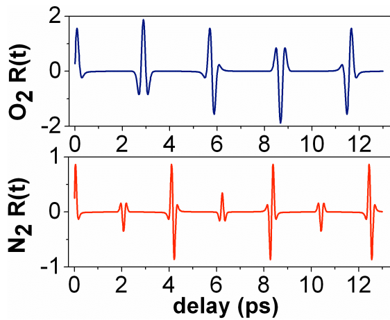
Fig. 2. Calculated response of the O 2 (top) and N 2 (bottom) molecules.
