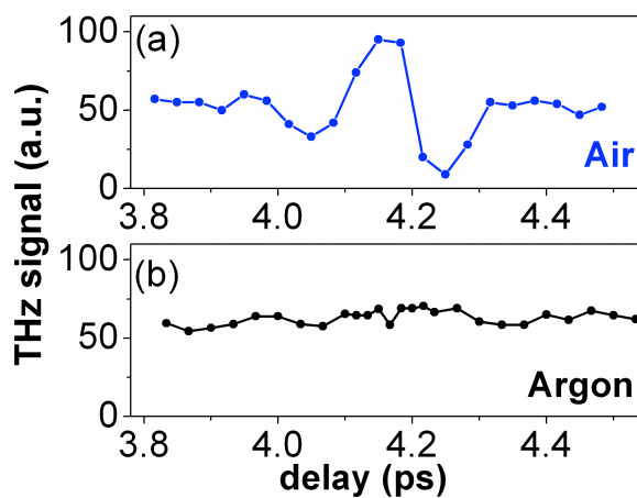
Fig. 3. THz intensity produced by bifilamentation as a function of the delay between the two laser pulses (pulse energy: 2 mJ; pulse duration: 50 fs) around the half-revival period of N 2 molecule in air (a) and in Argon (b). The enhancement factor of the THz radiation in case (a) is about 10.
