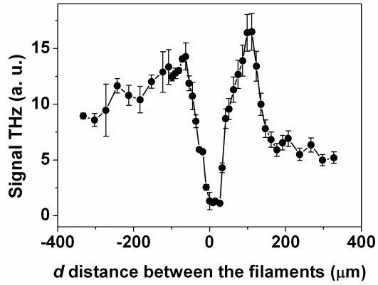
Fig. 1. THz intensity as a function of the distance between the two filaments. The two filaments were created by two laser pulses of 50 fs duration and 1.5 mJ energy. The maximum enhancement of the THz radiation is on the order of 30 as compared to a single filament.
