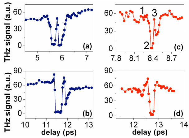
Fig. 4. (a) and (b), measurement of the variation of the THz intensity as a function of delay between the two laser pulses around the half and full revival period of O 2 . (c) and (d) show the same measurements in N 2 for time around 1 and 3/2 of the revival period. Enhancement of the THz radiation is about 20 for each figure.
