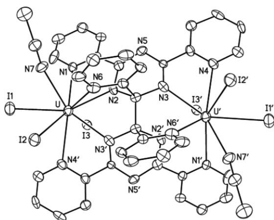
Fig. 3 View of 3 . The H atoms have been omitted. Displacement ellipsoids are drawn at the 20% probability level. Symmetry code: ' = 2 - x, y, 1/2 - z . Selected bond lengths (Å) and angles ( ^{\circ} ): U–N1 2.662(17), U–N2 2.412(16), U–N3' 2.466(19), U–N4' 2.660(18), U–N6 2.750(19), C13–C13' 1.49(4), C13–N2 1.51(3), C13–N3 1.45(3); N1–U–N2 63.2(6), N2–U–N3' 62.9(6), N3'–U–N4' 63.2(6), N1–U–N6 97.0(6), N2–U–N6 59.7(6), N3'–U–N6 73.5(6), N4'–U–N6 122.4(6).
