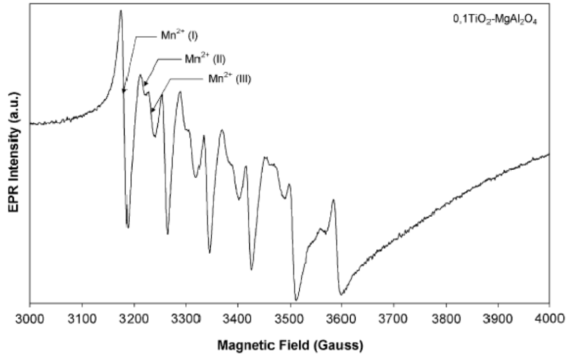
Fig. 1. EPR spectrum of the 0.1\text{TiO}_2\text{-MgAl}_2\text{O}_4 sample recorded with c -axis parallel to the direction of the applied magnetic field B_0 ( T = 5\text{ K} , \nu = 9.490\text{ GHz} , p = 0.01\text{ mW} ).
