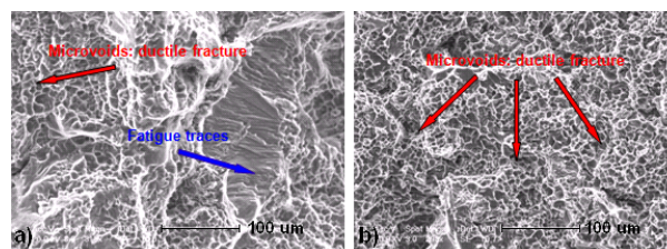
Figure 2 – Fracture faces taken in the Paris regime (regime II) of the crack growth for the test conducted at R=0.7/100^\circ\text{C}/20\text{Hz} ; a) at \Delta K \approx 5 \text{ MPa}\sqrt{\text{m}} ; b) at \Delta K \approx 7 \text{ MPa}\sqrt{\text{m}} .
