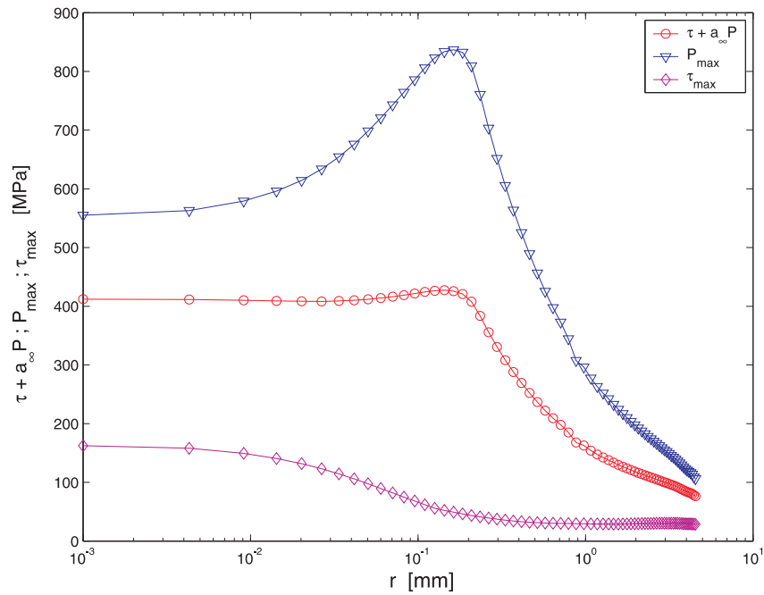
Figure 13. Distribution of the equivalent mesoscopic shear stress \tau + a_\infty P , the mesoscopic shear stress \tau and the hydrostatic pressure P along the bisector of the root of the LET for C_{up} = 433 \text{ Nm} and T = 113 \text{ kN} .
