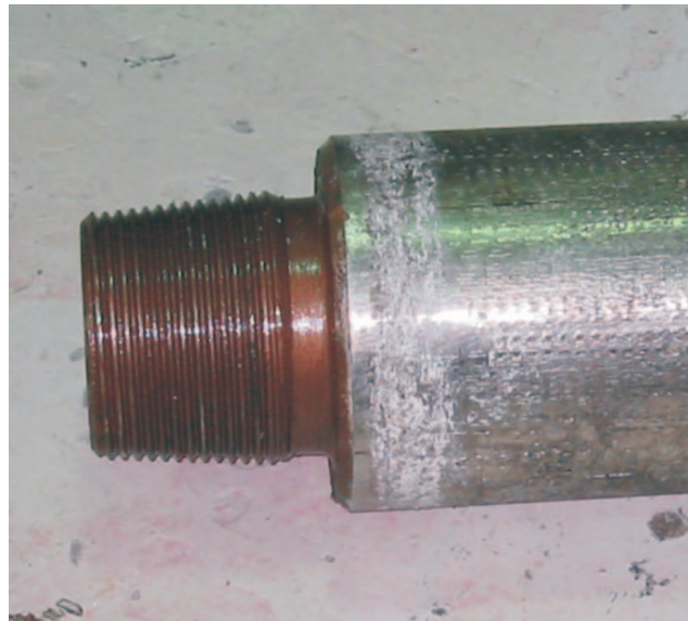
Figure 1. Description of a drillstring: a) drillstring components; b) picture of the pin part of a tool-joint.
