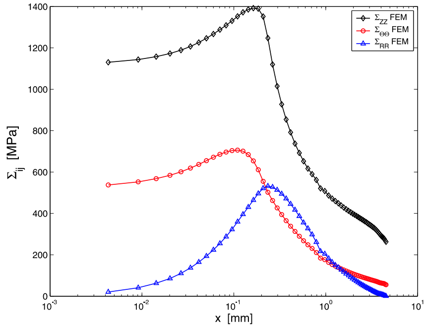
Figure 12. Stress distribution along the bisector of the root of the LET for C_{up} = 433 \text{ Nm} and T = 113 \text{ kN} .
