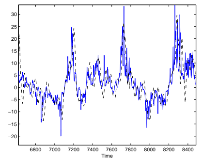
(c) Zoom of 7-(b)
