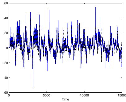
(b) SR_{100}(S\&P500) (-) and 10 days forecasting (- -)
