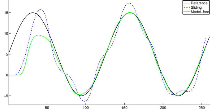
Fig. 8. Output tracking for both sliding mode and i-PID controllers
