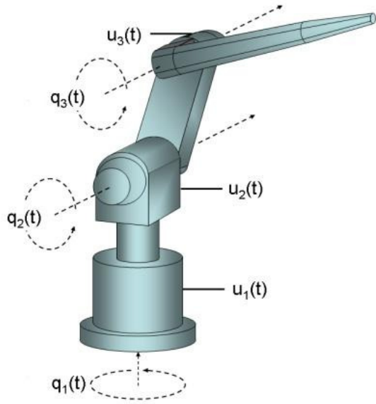
Fig. 14. Control inputs.
