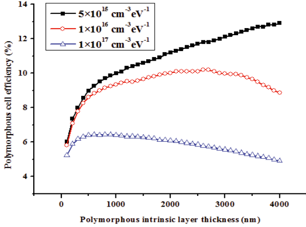
Fig. 2. Pm-Si:H cell efficiency as a function of pm-Si:H intrinsic layer thickness for three values of the Gaussian distribution peak value D_{\max} (expressed in \text{cm}^{-3} \text{eV}^{-1} ): 5 \times 10^{15} (■), 1 \times 10^{16} (○) and 1 \times 10^{17} (△).
