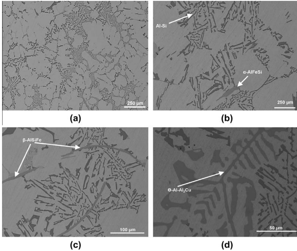
Fig. 1. Initial microstructure of LFC A319 (DAS = 73.3 μm): (a) global view of different phases, (b) Al-Si eutectics and α-AlFeSi intermetallic, (c) β-AlFeSi needle-like intermetallics, and (d) θ - Al - Al 2 Cu eutectics.
