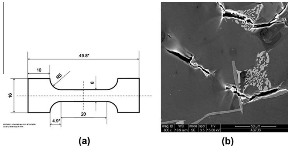
Fig. 6. In situ tensile test at room temperature, \Delta\epsilon = 0.45\% (a) specimen geometry and (b) crack path following brittle eutectic/intermetallic phases.
