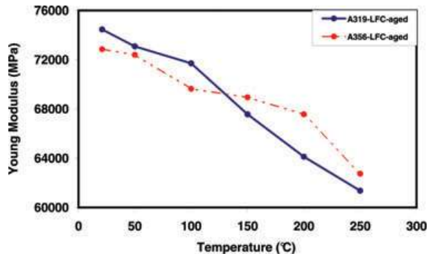
Fig. 6 Evolution of the Young Modulus E as a function of temperature for the aged A319 and A356 alloys.
