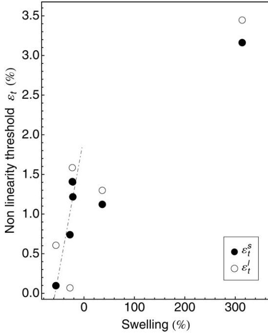
Figure 9. Nonlinearity thresholds \epsilon_t^s and \epsilon_t^l according to swelling degree.
