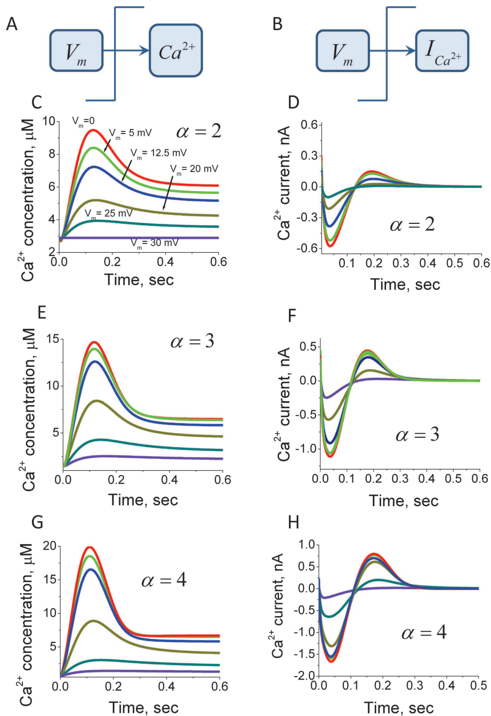
Figure 3 Systems model predictions for intraciliary Ca^{2+} concentration and current responses to the transmembrane potential shift.
