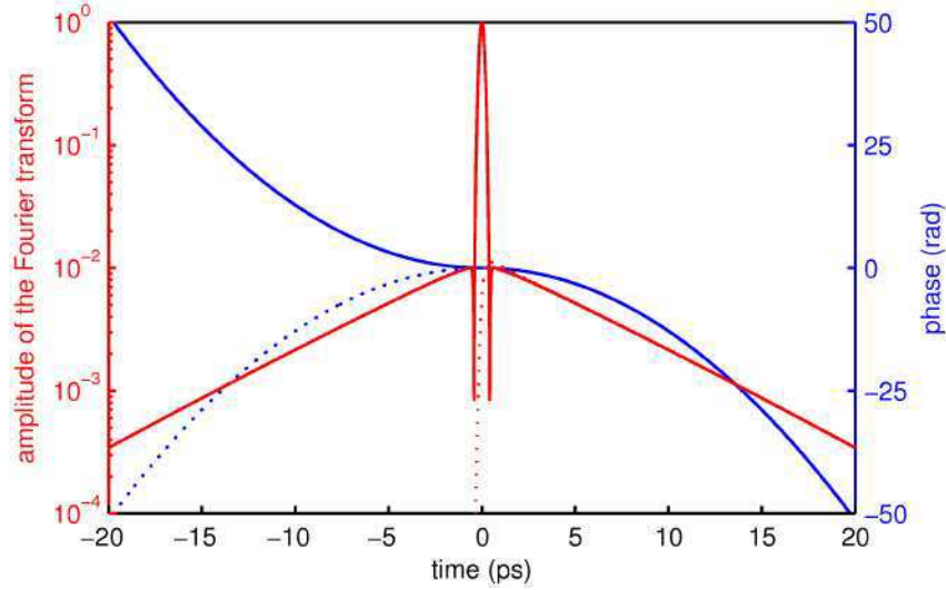
Fig. 2. The solid red line (left vertical axis) shows the amplitude of the Fourier transform of the spectral intensity, |[FT I_{cpu}(\omega)](t)| , with the same parameter values as in Fig. 1. The red dotted line shows the contribution of the second term of Eq. (4). The dotted blue line (right vertical axis) shows the time-dependent phase \Phi(t) of the chirped pulse. The solid blue line shows the time-dependent phase \Phi_{corr}(t) used in the data processing.
