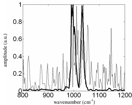
Fig. 5. Controlled homodyne (solid) and standard FTCARS (dashed) spectra of pyridine using 5mW pump and 5 mW probe power.
