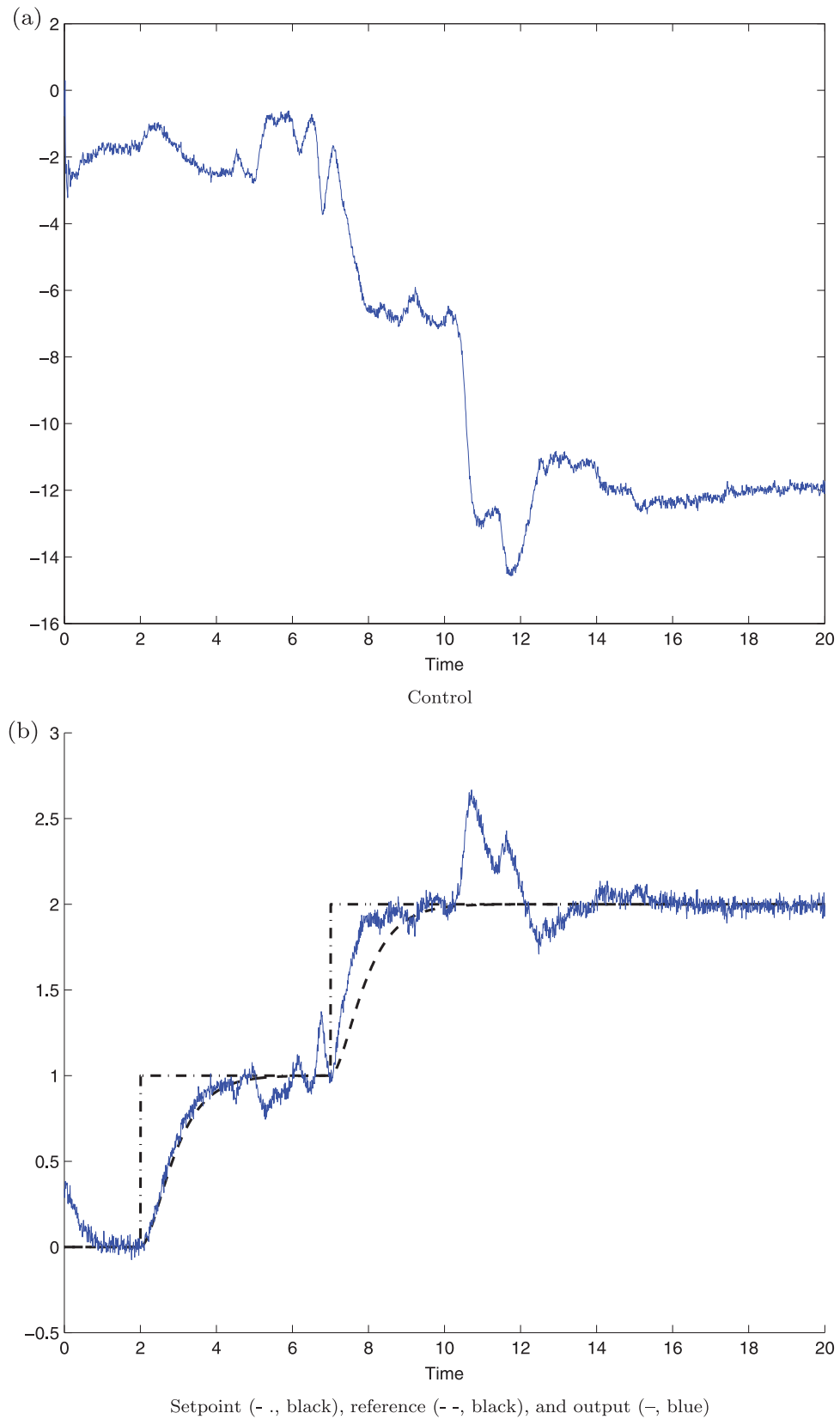
Figure 11. Delay system: Model-free control. (a) Control. (b) Setpoint (· · ·, black), reference (---, black), and output (—, blue).
