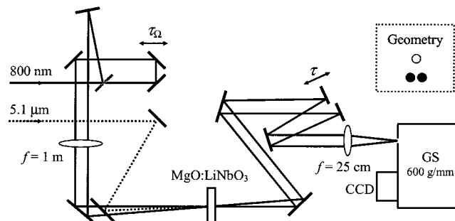
Fig. 1. Upconversion and ZAP SPIDER apparatus. Two chirped 800-nm pulses (5 \mu\text{J} each, 150 ps) are derived from the zero-order diffraction of the CPA compressor and mixed noncollinearly with the 1- \mu\text{J} mid-IR pulses in a 425- \mu\text{m} MgO:LiNbO 3 crystal. The signals are imaged on the slit (set at 8 \mu\text{m} ) of a grating spectrometer (GS). Inset, upconversion beam geometry of mid-IR (white) and stretched (black) pulses.
