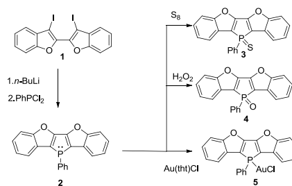
Scheme 1: Synthetic routes to furan-phosphole derivatives 2-5
