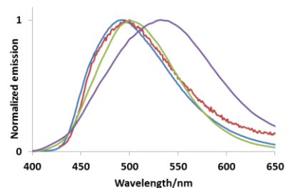
Figure 4: Photoluminescence of 4 in solution (CH 2 Cl 2 , 10 -5 M) (blue) and in the solid state (red); Electroluminescence of device B (green) and device A (purple).
