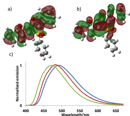
Figure 3: a) HOMO of 4 , b) LUMO of 4 , c) Normalized emission spectra in CH 2 Cl 2 of 3 (red), 4 (blue) and 5 (green).
