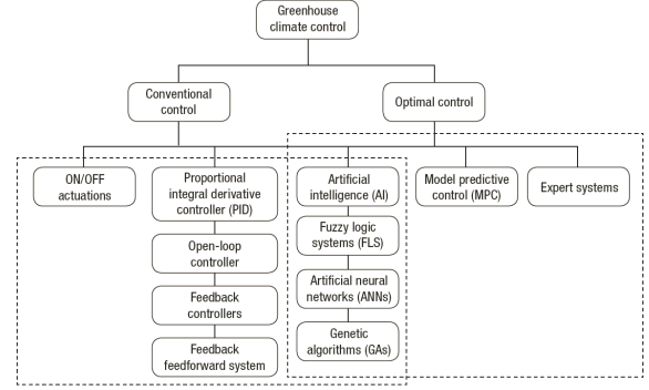
Fig. 1. Greenhouse control theories classification
