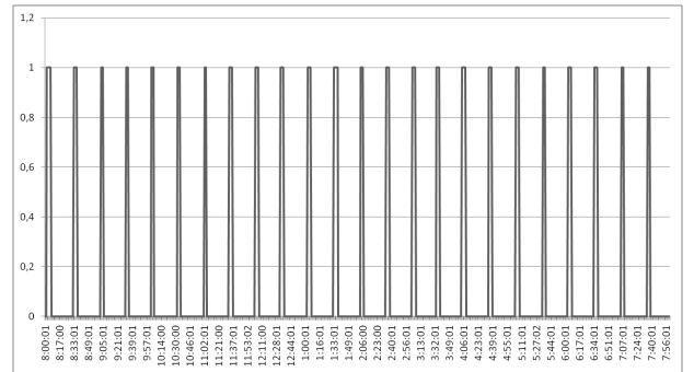
Fig. 12. Fog control with a Boolean controller
