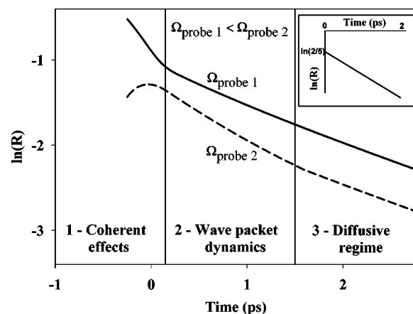
FIG. 2. Schematic presentation of R in presence of rotation–vibration coupling effects. The insert reproduces the results of the simple theory. Coherent effects dominate in the time domain 1, wave packet dynamics governs the time domain 2, whereas rotational diffusion is characteristic of the time domain 3. In this figure \Omega_{\text{probe } 1} and \Omega_{\text{probe } 2} represent two values of the probe frequency \Omega_{\text{probe}} .
