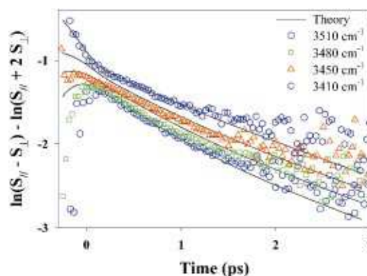
FIG. 4. (Color) Rotational anisotropy R measured experimentally (symbols \square , \circ , \triangle , \diamond ), and calculated theoretically (full curves). The pump frequency \Omega_{\text{pump}} is equal to 3510 \text{ cm}^{-1} , and the probe frequencies \Omega_{\text{probe}} are equal to 3510 , 3480 , 3450 , and 3410 \text{ cm}^{-1} , respectively.
