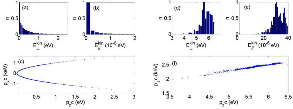
FIG. 4. Histograms of calculated kinetic energies of free electrons born during filamentation in the transverse and longitudinal directions with respect to the filament axis z . (a-b) relate to linearly polarized laser light and (d-e) to circularly polarized light. Also shown are p_x^c the transverse and p_z^c the longitudinal components of the drift momentum for (c) linearly and (f) circularly polarized pulses. The perpendicular momentum for circular polarization corresponds to p_{\perp} = \sqrt{p_x^2 + p_y^2} .
