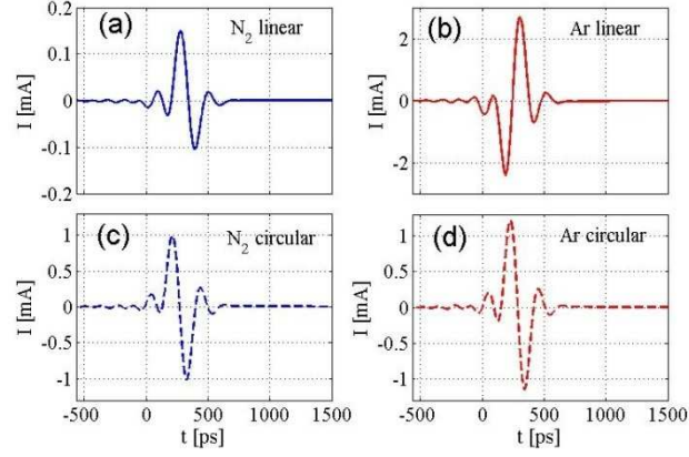
FIG. 2. Current signal (after deconvolution from the detection response function) measured in N_2 (left) and Ar (right) as a function of laser polarization. Upper traces are obtained with linearly polarized light, lower traces with circularly polarized light. The laser pulse has duration of 35 fs and energy of 2 mJ.
