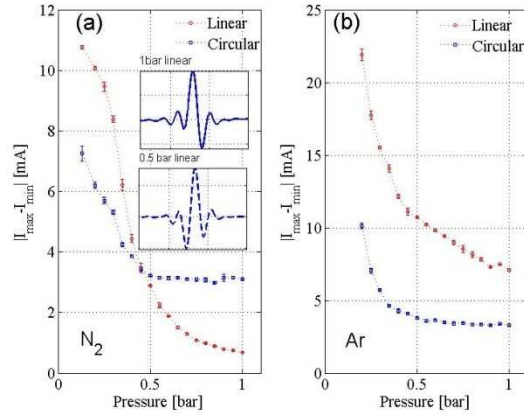
FIG. 3. Amplitude of the current measured by the induction coil in N_2 (left) and Ar (right) as a function of gas pressure for linearly and circularly polarized light. The laser pulse has a duration of 35 fs, an energy of 3 mJ and is focused with a lens F = 100 cm. Filamentation occurs above 400 mbar. Also shown in the inset are the current signals in N_2 for 1 bar (top) and 0.5 bar (bottom).
