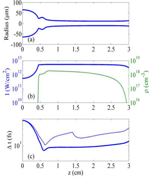
FIG. 4. Calculated results of the propagation through fused silica of an optical pulse at 1.9 \mu\text{m} of 110 \mu\text{m} diameter (FWHM) and 5 \times 10^{11} \text{W}/\text{cm}^2 intensity collimated on the front sample surface. a) Beam radius as a function of distance z . b) Intensity (full line) and free electron density (dotted green line) as a function of z . c) Pulse duration as a function of z . The blue line corresponds to the duration within the filament core of 25 \mu\text{m} diameter, the red line corresponds to the duration obtained when averaging over a filament diameter of 50 \mu\text{m} .
