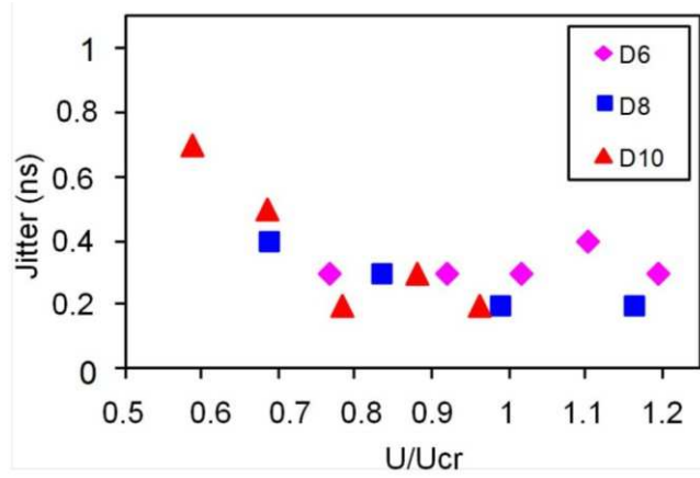
FIG. 4. (Color online) Jitter for the gap switch with the hole \varnothing 3 mm and gaps 6 (D6) to 10 (D10) mm.
