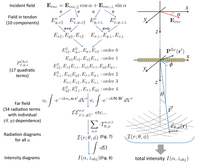
FIG. 5. (Color online) Data flow of PSHG numerical calculation. For two components E_{inc,\parallel} and E_{inc,\perp} of the incident field, ten components E_{i,\parallel,\perp}^{o,e} of the focal field are calculated in the tendon. The induced nonlinear polarization \mathbf{P}_i^{2\omega} then contains 17 quadratic terms of different order and symmetry. Each of these terms produces an ordinary \mathcal{E}^o and an extraordinary \mathcal{E}^e radiation component (34 total). Radiation diagrams \mathcal{I}(\theta, \varphi) for any chosen \alpha are then calculated using these components \mathcal{E}\mathcal{E} and their respective angular dependences T_{\theta,\varphi}^{o,e,i} . Integration of \mathcal{I}(\theta, \varphi)|_{\alpha, z_{obj}} over the solid angle of radiation produces intensity diagrams I(\alpha, z_{obj}) .
