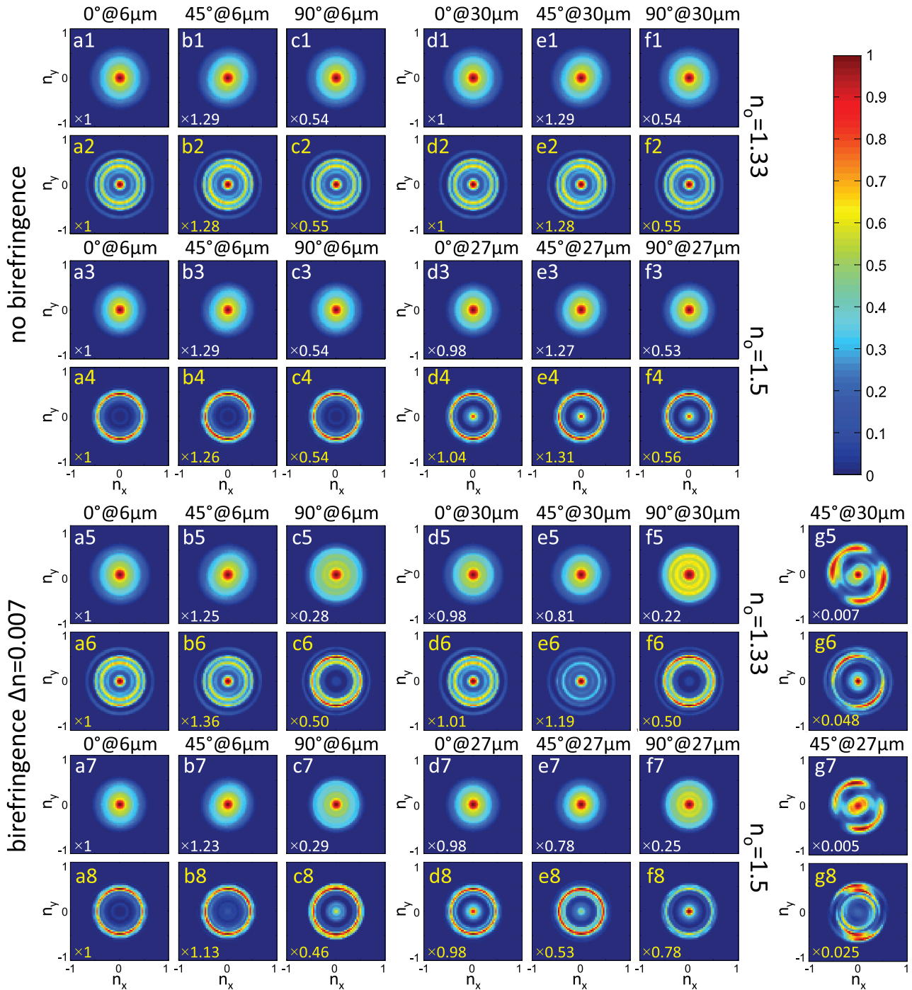
FIG. 7. (Color online) Simulated SHG radiation angular diagrams \mathcal{I}(n_x, n_y) as functions of n_x = \sin \theta \cos \varphi and n_y = \sin \theta \sin \varphi for the eight parameter sets listed in Table I and for two different imaging depths z_{\text{obj},1} and z_{\text{obj},2} . z_{\text{obj},1} was set to 6 \mu\text{m} and corresponds to the imaging plane in the proximity of the tendon-water interface. z_{\text{obj},2} corresponds to the depth where the phase shift between the incident squared fields (E_x^\omega)^2 and (E_y^\omega)^2 attains \pi : 30 \mu\text{m} for n_o = 1.33 and 27 \mu\text{m} for n_o = 1.5 . Intensities within a set (a)–(g) are normalized to the maximal intensity in (a), and relative intensities are shown in the bottom left corner as a multiplying coefficient ( \times \dots ). Diagrams (a) are for the incident field polarized at \alpha = 0 to the tendon axis, at the depth z_{\text{obj},1} , (b) for \alpha = \pi/4 , z_{\text{obj},1} , (c) for \alpha = \pi/2 , z_{\text{obj},1} , (d) for \alpha = 0 , z_{\text{obj},2} , (e) for \alpha = \pi/4 , z_{\text{obj},2} , and (f) for \alpha = \pi/2 , z_{\text{obj},2} . (g) Radiation diagrams created by P_x^{2\omega} at z_{\text{obj},2} at the angle \alpha for which maximal intensity extinction is obtained ( \alpha shown at the upper right corner). These diagrams (g) are not observed directly.
