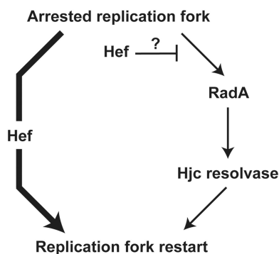
Figure 7. Model for replication restart in H. volcanii . Two alternative pathways allow replication restart: one is dependent on the homologous recombination proteins Hjc and RadA (pathway on the right) and one is independent of homologous recombination (pathway on the left). Our data show that Hef has a dominant role during replication restart, even in the presence of Hjc, and are also compatible with Hef, preventing the access of recombination proteins at arrested forks.
