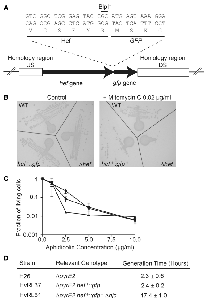
Figure 1. gfp -fused hef allele construction and functional characterization. (A) Representation of the chromosomal locus of the hef :: gfp allele. The regions of homology between the plasmid and the chromosome used for pop-in/pop-out gene replacement are represented by white boxes (Upstream region and downstream region). The sequence of the 3' end of the H. volcanii hef gene fused to the gfp gene is shown. BlnI* refers to the inactivated restriction site after cleavage and processing of the cohesive extremity into blunt end. (B) Strains streaked on YPC control plates and YPC plates containing 0.02 µg/ml MMC after 7 days of incubation. (C) Fraction of living cells in response to increasing concentrations of aphidicolin for WT (black square), hef -deleted (black triangle) and hef + :: gfp + cells (black circle). Error bars represent standard deviations of at least three independent experiments. (D) Generation times (± SEM) of WT and hef + :: gfp + cells, and hef + :: gfp + in a hjc -deleted background.
