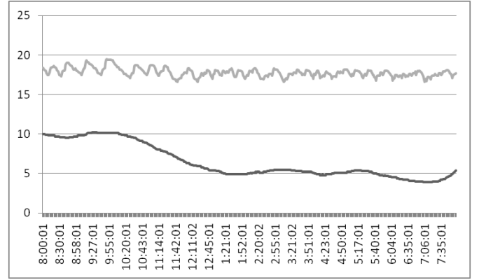
Fig. 12. Internal temperature with model-free control (Te: Black line - Ti: Grey line)
