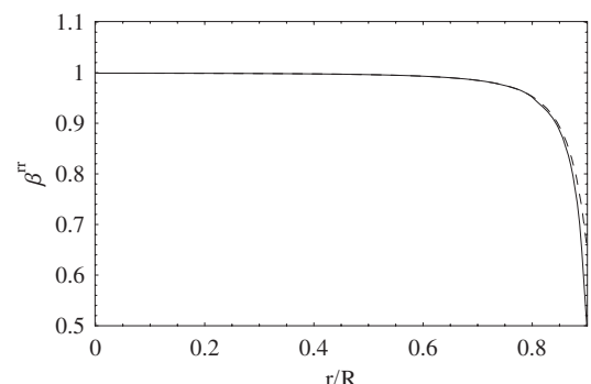
FIG. 5. Plot of \tilde{\beta}^{rr}(r) as a function of r/R for a = 0.1 R , exact (solid) and approximate (dashed). The exact function vanishes at r = R - a .
