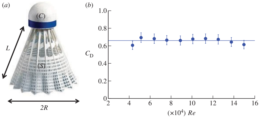
Figure 6. (a) Geometrical characteristics of a shuttlecock. (b) Evolution of the drag coefficient, C_D = 2F_D / \rho \pi R^2 U^2 , of a shuttlecock with the Reynolds number Re = 2RU/v . (Online version in colour.)
