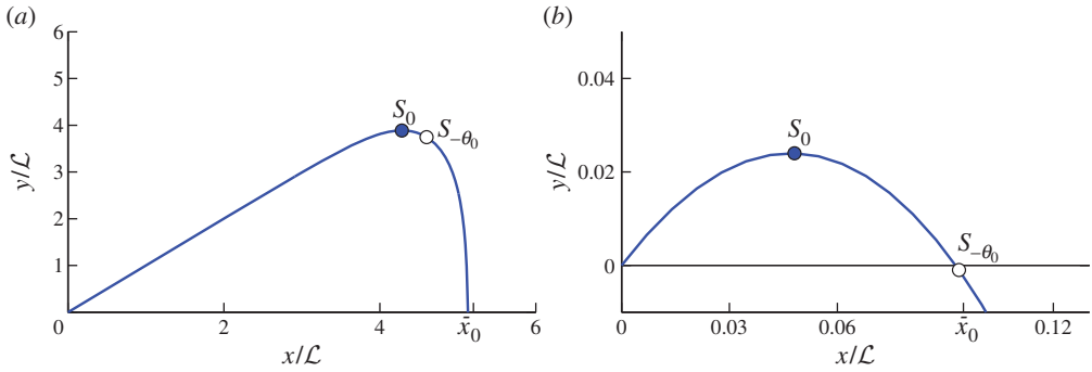
Figure 12. (a) Trajectory obtained from the numerical integration of (4.12) with \theta_0 = \pi/4 and (U_0/U_\infty)^2 = 10^5 . (b) Trajectory obtained from the numerical integration of (4.12) with \theta_0 = \pi/4 and (U_0/U_\infty)^2 = 0.1 . (Online version in colour.)
