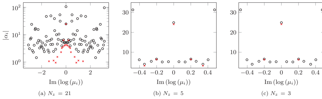
FIG. 16. (a) N_z = 21 , (b) N_z = 5 , (c) N_z = 3 : Dependence of the absolute value of the amplitudes \alpha_i on the frequency (imaginary part) of the corresponding eigenvalues \mu_i for the flow through a cylinder bundle. The results are obtained using the standard DMD algorithm (circles) and the sparsity-promoting DMD algorithm (crosses) with N_z DMD modes.
