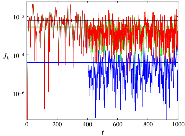
FIGURE 7. Cost functional J = \mathcal{E}(y^2 + lu^2) as a function of time without control (in black) and with control applied (in green, red and blue). The blue line represents full-state control designed from knowledge of all full-order system matrices as well as q . The green line represents LQG control designed from the full-order system matrices and noise covariances (same as in figure 3b). The red line is the cost functional based on LQG control designed from the identified model and the identified noise covariances. In addition to the cost functional J the quantity J_k = y_k^2 + lu_k^2 is displayed. The control is switched on at t = 400 , and a convection velocity of U_r = 3 is chosen.
