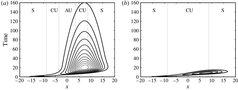
FIGURE 1. Response to an impulse from the noise location shown as |q| contours in an x - t diagram: (a) for a moderate convection speed U_r = 2 and (b) for a large convection speed U_r = 3 . The absolutely unstable (AU), convectively unstable (CU) or stable (S) spatial domains are marked.
