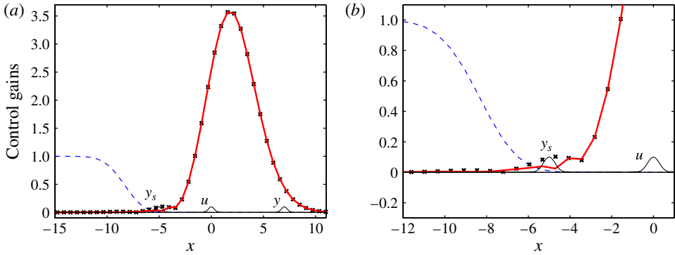
FIGURE 24. (Colour online) The control gains \mathbf{K} and \bar{\mathbf{K}} designed from \mathbf{A} (full line; red online) and from \mathbf{A} - \mathbf{L}\mathbf{C}_s (crosses), respectively, are compared, as a function of x . On the same plot the relative estimation error is presented as a dashed line. Panel (b) is a zoom of panel (a), focusing on the spy sensor location.
