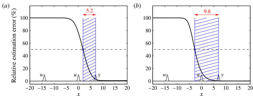
FIGURE 9. (Colour online) Ratio of the standard deviation of the estimation error to the standard deviation of the state as a function of streamwise position x for a convection speed of (a) U_r = 3 and (b) U_r = 2 . In both figures, the visibility length (see text) has been added.
