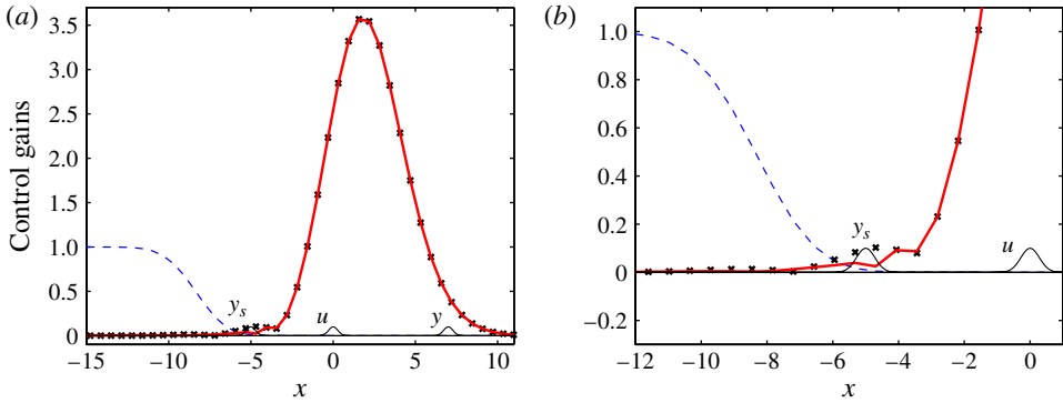
FIGURE 24. (Colour online) The control gains K and \bar{K} designed from A (full line; red online) and from A - LC_s (crosses), respectively, are compared, as a function of x . On the same plot the relative estimation error is presented as a dashed line. Panel (b) is a zoom of panel (a), focusing on the spy sensor location.
