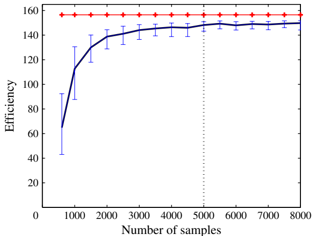
FIGURE 26. (Colour online) Control efficiency of the feed-forward approach as a function of the number of samples for the complex Ginzburg–Landau model. Fifty realizations of identification and control were performed; the average (full line with error bars; blue online) and the standard deviation are displayed. These curves are compared to the optimal LQG control designed from the full-order system (full line with plus symbols; red online).
