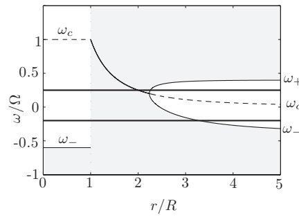
FIG. 16. Epicyclic frequencies \omega_+ and \omega_- (thin solid lines) and critical frequency (thin dashed lines) as a function of r for f/\Omega = -0.4 for m = 1 . Dotted lines represent the boundary of the vortex core. The two thick solid lines show examples of the frequency \omega_r for the upper and lower neutral branches in Fig. 14. The regions where the WKB approximations are wavelike (i.e., \Delta < 0 ) are shaded.
