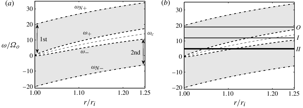
FIGURE 3. Typical example of the sign of \beta for the same parameters as in figure 1. The epicyclic frequencies \omega_{\pm} and the critical frequencies \omega_{N\pm} are plotted by thick dashed and thick dot-dashed lines, respectively. The critical frequency \omega_c = m\Omega at which s = 0 is also plotted by dashed lines. The regions where the solutions are wavelike ( \beta > 0 ) are shaded. Panel (b) is the same as panel (a) except that solid lines show examples of the frequency \omega_r for which there is no turning point (O), one turning point (I) or two turning points (II).
