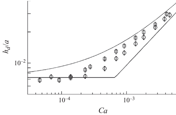
FIGURE 4. Deposited thickness as a function of Ca , for two different pillar spacings: d = 10 \mu\text{m} (squares) and d = 20 \mu\text{m} (circles), and comparable pillar height h_p (9.8 and 11 \mu\text{m} , respectively). We also represent two asymptotic behaviours: the low pillar density limit, h_d = \max(h_p, h_{LLD}) (solid line), and the high pillar density limit, h_d = h_p + h_{LLD} (dotted line).
