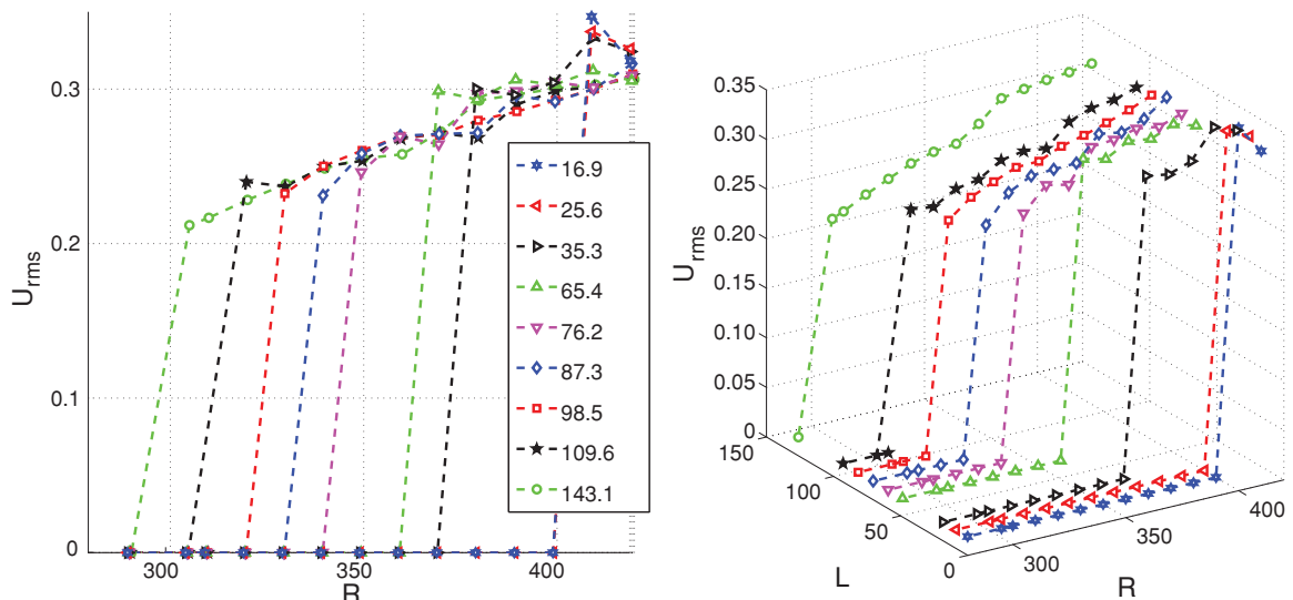
FIG. 11. (Color online) (a) Bifurcation diagrams in the R - D plane for the different system sizes indicated in the legend, with D \equiv U_{\text{rms}} . (b) Three-dimensional unfolding of (a) according to system size L .
