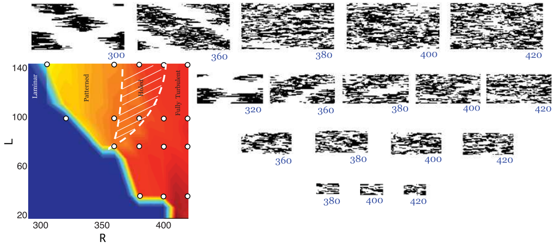
FIG. 12. (Color online) Left: Bifurcation diagram in the R - L plane with color coded values of D \equiv U_{\text{rms}} ; red (rendered medium gray) corresponds to the largest value of D (turbulent at large L , chaotic at small L ); blue (rendered dark gray) is for laminar flow where D = 0 ; patterns and rigged states have intermediate values of D from yellow to orange (rendered light to medium gray). Above and on the right: BW representation of turbulent-laminar patches for L = 143.1 (top), 98.5 , 76.2 , and 35.3 (bottom). Corresponding Reynolds numbers are indicated at the bottom right corner of each image. White dots in the left panel show the location of the states corresponding to the BW plots. Cases ( L = 143.1 , R = 300 ) and ( L = 98.5 , R = 320 ) are decaying and eventually become laminar.
