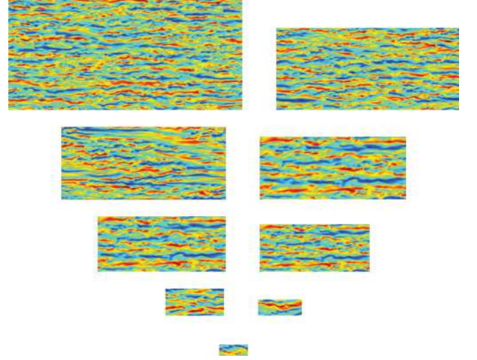
FIG. 3. (Color online) Streamwise velocity fluctuations ( u ) in the plane y = 0 for different domains at R = 410 : L = 143.1 (top left), 109.6 (top right), 98.5, 87.3, 76.2, 65.4, 35.3, 25.6, and 16.9 (bottom).
