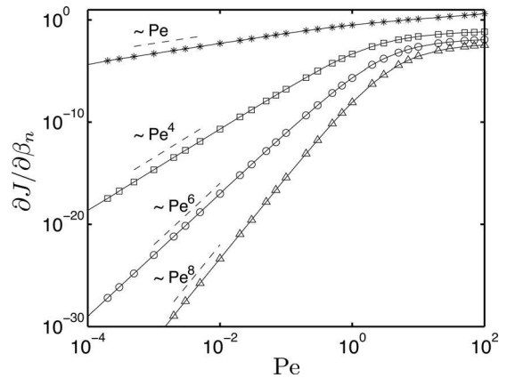
FIG. 6. Dependence with the Péclet number, Pe , of the nutrient flux gradient \partial J / \partial \beta_n with respect to the first four odd modes n = 1 (stars), n = 3 (squares), n = 5 (circles), and n = 7 (triangles) and evaluated at the treadmill (the even mode gradients are equal to zero by symmetry). The power law dependence of each component is indicated by a dashed line.
