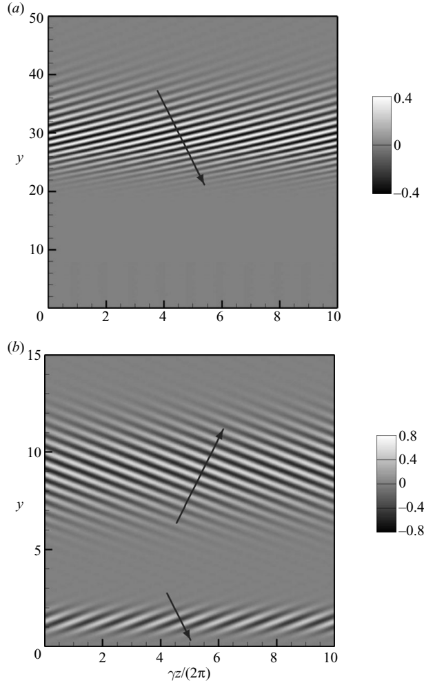
FIGURE 16. Disturbance fields of the algebraically decaying eigenmodes for (a) \lambda = (1.5 - 0.1i)\gamma and (b) \lambda = (0.7 - 0.4i)\gamma . The arrows indicate the dominant direction of the wave propagation. ( \gamma = 0.3 , R = 1000 ).
