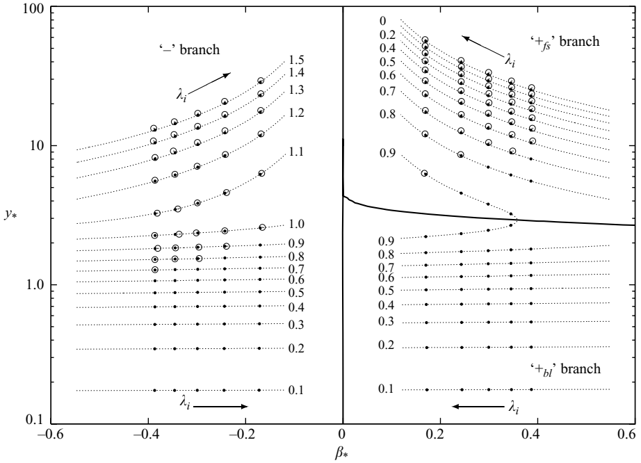
FIGURE 12. Location of the peak and the wavenumber of the numerically evaluated wave packet pseudo-mode (○) compared to the values predicted by the symbol (●). The dotted curves are lines for which \lambda_r/\gamma is constant (the value of \lambda_r/\gamma is indicated next to the curves). The dots indicate different values of the imaginary part \lambda_i/\gamma = -0.5, -0.4, -0.3, -0.2, -0.1 . The solid line defines the border of the region for which the twist condition is satisfied ( \gamma = 0.3, R = 1000 ).
