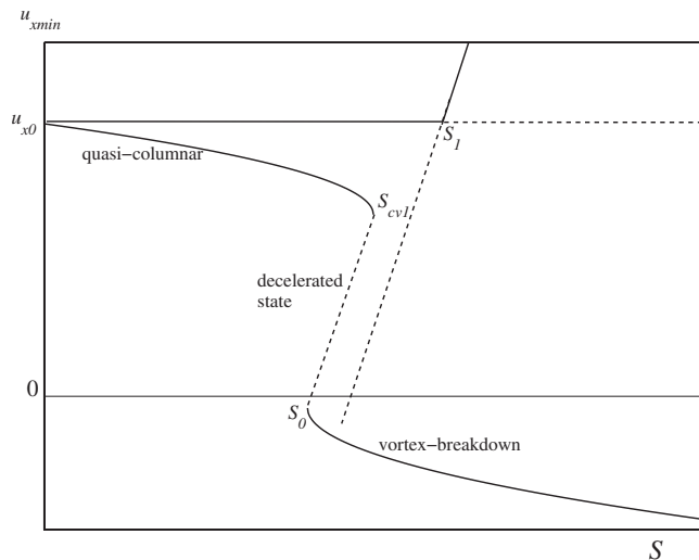
FIG. 1. Qualitative bifurcation diagram for axisymmetric vortex breakdown for both inviscid and viscous flows. Here, u_{xmin} is the minimum axial velocity found at any point in the computational domain.
