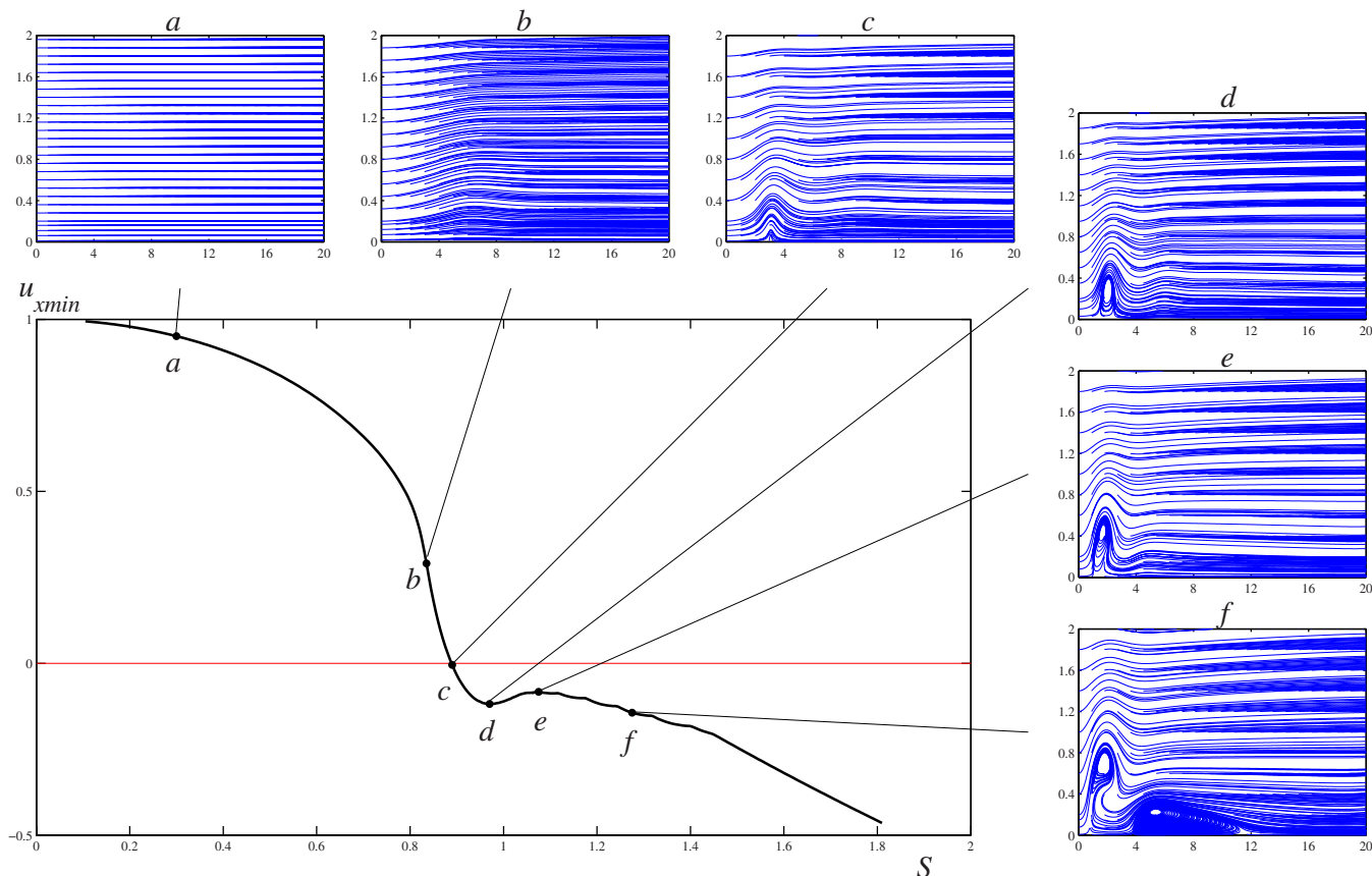
FIG. 2. (Color online) Bifurcation diagram describing the formation of vortex breakdown as the swirl is increased. The minimum axial velocity u_{x\min} is plotted as a function of the swirl number S for Re=200 . Each point along the bifurcation curve corresponds to a steady-state solution of the Navier–Stokes equations. The streamlines of some of the corresponding characteristic steady states are shown on the top and on the right. The wiggles on the bifurcation diagram visible after S=1 are converged (i.e., identical when the resolution is increased); they disappear when a less specific measure is taken as, for example, the overall mean value of u_x .
