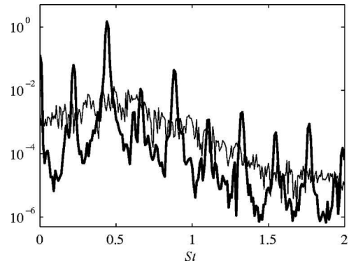
FIG. 3. Spectral density of v'(r=1, x=1, t) as a function of Strouhal number for the two configurations of Fig. 2. Thin line: globally stable case R/\theta=25 , S=0.65 ; thick line: globally unstable case R/\theta=25 , S=0.55 .
