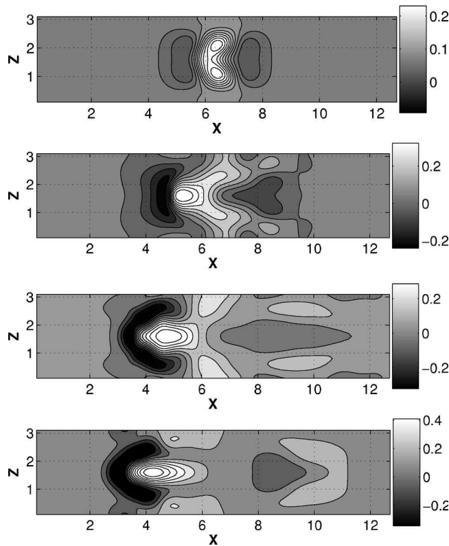
FIG. 8. Generation and entrainment of a crescent vortex, depicted by its vertical velocity V_1 . From top to bottom, t=0.1, 1, 3, and 5 . The flow field (U_1, W_1) is given below in Fig. 9.
