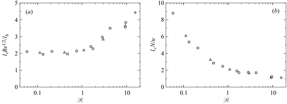
FIGURE 11. The scaled vertical length scale (a) l_v Re^{1/2} / l_h and (b) l_v N / u as a function of R . Circles, runs A; triangles, runs B; diamond, run C; squares, runs D.
