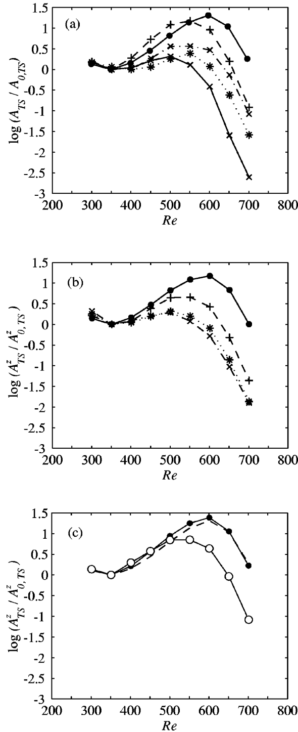
FIG. 18. Alternative amplitude measures. (a) shows the maximum measure, (b) the y -integral measure, and (c) the z -integral measure. The different symbols correspond to R case (●); S 2 case (+) high speed, (*) shear, (×) low speed, and (○) the spanwise integrated. Dash-dotted and solid lines of (×) correspond to outer and inner peaks, respectively, and other lines are for visual aid only. See text for dashed line in (c). F = 130.
