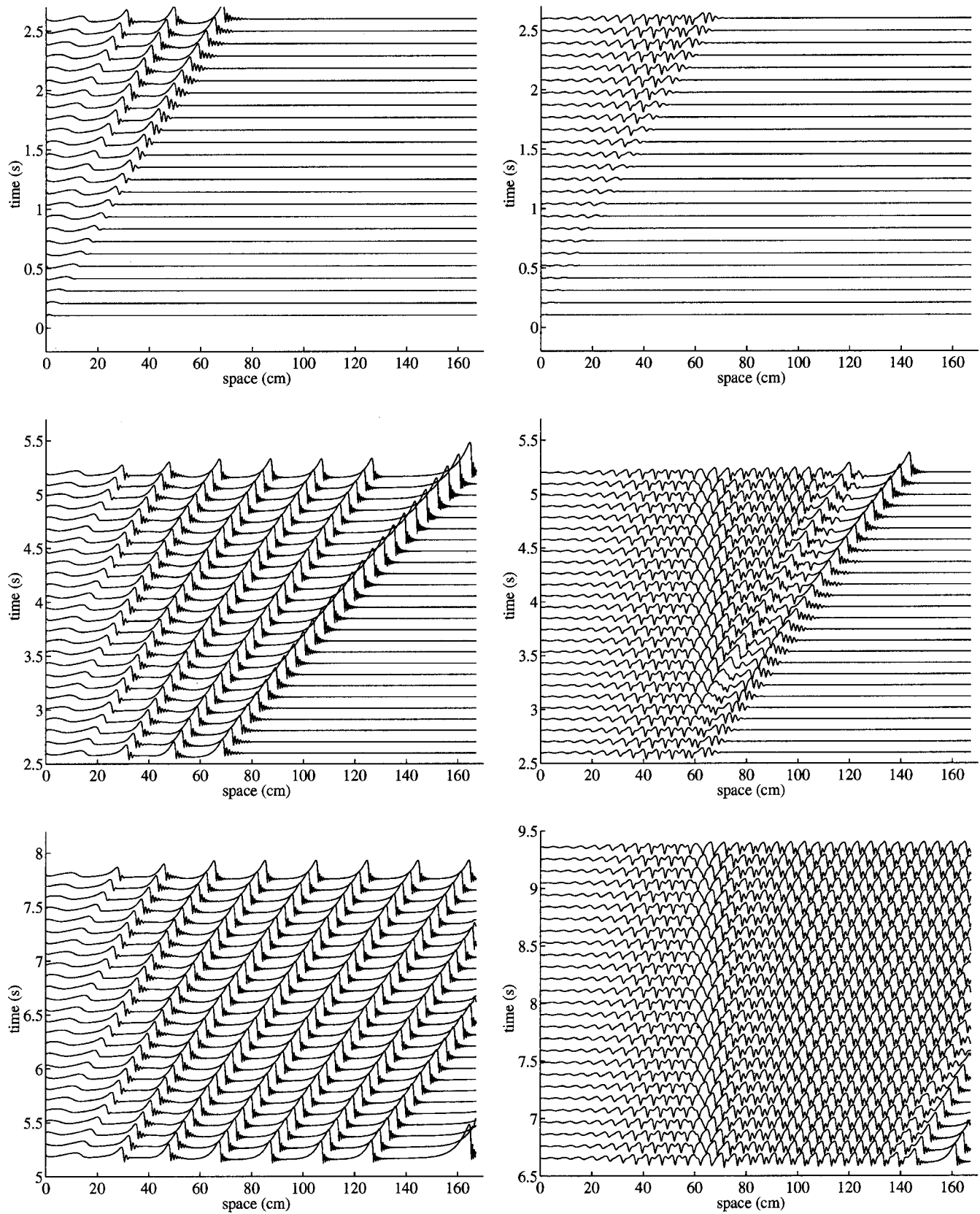
FIG. 8. Film thickness evolution in the experimental conditions of Liu and Gollub (Ref. 13). Left: f=1.5 Hz, A=0.15 . Right: f=4.5 Hz, A=0.03 . For comparison with Figs. 14 and 16 in Ref. 14, respectively.
