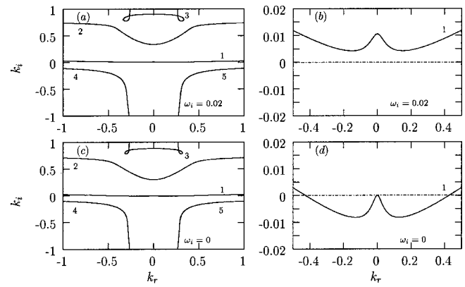
FIG. 2. Spatial branches k_n in the (k_r, k_i) plane for dispersion relation (19) with \omega_i = 0.02 (top) and \omega_i = 0.0 (bottom). R = 40 , \beta = 4.6^\circ , W = 41.46 ( \Gamma = 769.8 ). Left: overall view of the diagram. Right: zoom on the neighborhood of the origin in the complex k plane.
