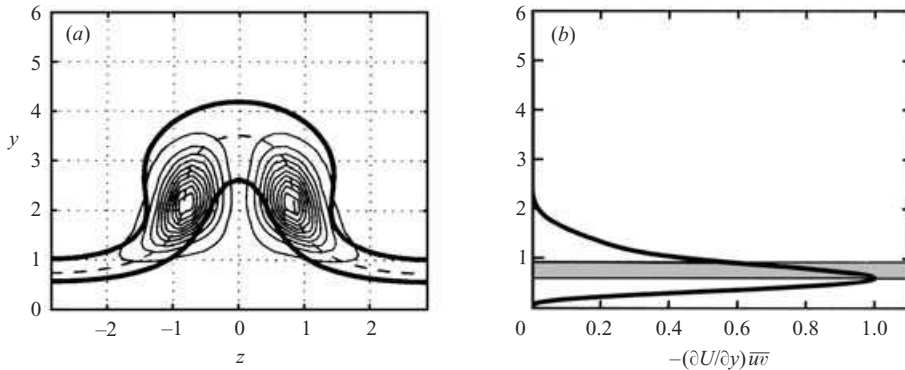
FIGURE 7. Production of perturbation kinetic energy and wave packet characteristic velocities. (a) Contour levels (thin solid lines) of the total production density -(\partial U / \partial y) \overline{uv} - (\partial U / \partial z) \overline{uw} in a cross-stream (y, z) -plane for the impulse response of the streaky base flow of figure 1(b). The outer contour is 5% of the maximum and contour spacing is 10% of the maximum. The thick solid lines represent the base flow velocity contours U(y, z) = v^+ and U(y, z) = v^- with v^+ = 0.935 and v^- = 0.66 . The dashed line represents the base flow velocity contour U(y, z) = v^{max} with v^{max} = 0.80 . (b) Wall-normal profile (thick solid line) of the production density -(\partial U / \partial y) \overline{uv} for the impulse response of the Blasius base flow. The grey horizontal strip delineates the region of base flow velocities v^- < U_B(y) < v^+ with v^+ = 0.5 and v^- = 0.36 .
