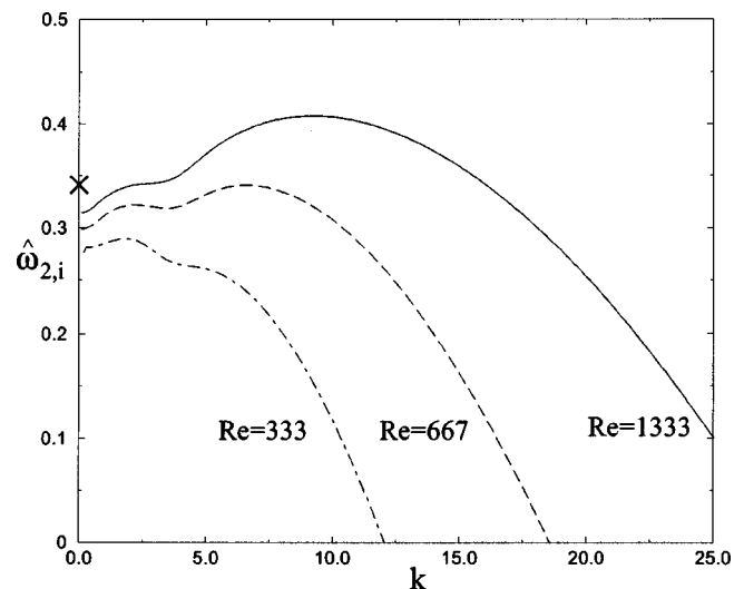
FIG. 5. Growth rate \hat{\omega}_{2,i} of the m=2 mode as a function of k for \alpha=5 and different Reynolds numbers: \text{Re}=1333 (continuous line), \text{Re}=667 (dashed line), and \text{Re}=333 (dashed-dotted line).
