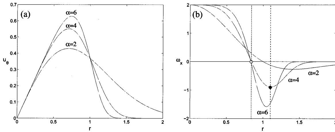
FIG. 1. (a) Dimensionless azimuthal velocity profiles u_\theta(r) for various \alpha=2, 4 , and 6 ; (b) dimensionless axial vorticity profiles \omega_x(r) for the same values of \alpha . For \alpha=4 , the filled circle corresponds to the locus of a minimum in axial vorticity signaling an eventual azimuthal shear instability and the open circle corresponds to the radius where the axial vorticity becomes negative and Rayleigh's criterion applies.
