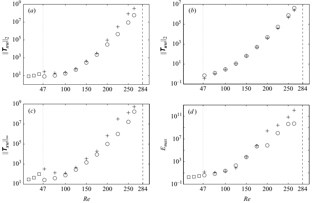
FIGURE 4. Performance of the uncontrolled ( \square , Re < 47 ) and controlled linear wake model as a function of Reynolds number for two control penalties (+) \ell = 1000 , ( \circ ) \ell = 0.1 using full information \mathcal{H}_2 control. (a) Transfer function 2-norm \|\mathbf{T}_{xw}\|_2 ; (b) transfer function 2-norm \|\mathbf{T}_{uw}\|_2 ; (c) transfer function \infty -norm \|\mathbf{T}_{xw}\|_\infty ; (d) maximum transient energy growth E_{max} . All plots are semilog-y and were computed using double precision arithmetic; note that, at this precision, stabilizing linear control feedback could not be determined above Re \approx 284 .
