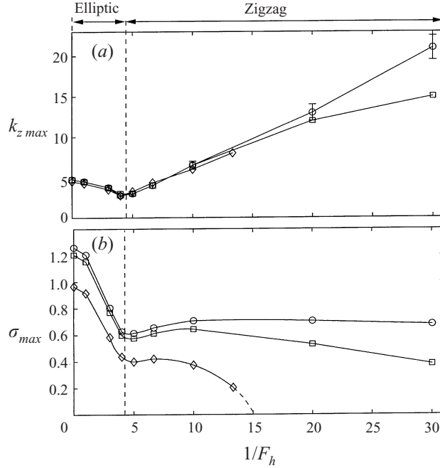
FIGURE 2. (a) Wavenumber k_{z\max} and (b) growth rate \sigma_{\max} of the fastest growing perturbation as a function of the inverse Froude number. \circ , \{Re = 10000, Sc = 1\} ; \square , \{Re = 1000, Sc = 1\} ; \diamond , \{Re = 200, Sc = 637\} . In (a), the error bars indicate the indeterminacy on the estimation of k_{z\max} resulting from the discretization of k_z . The regimes labelled Elliptic and Zigzag indicate the regions where the instability is of elliptic type and of zigzag type, respectively.
