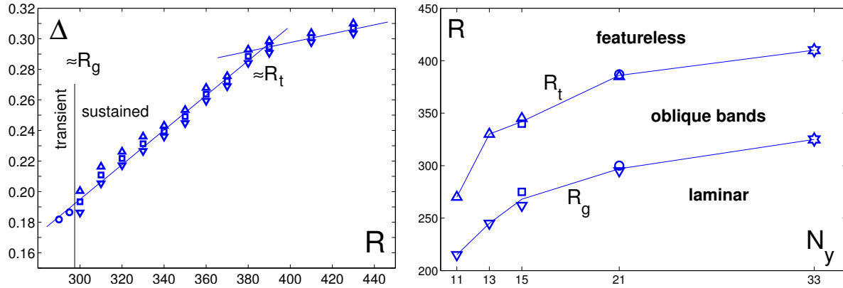
Figure 1. Variation of the time-average of the distance \Delta to laminar flow as a function of R for N_y = 21 with (L_x, L_z) = (110, 84) and (N_x, N_z) = (440, 336) , see (Manneville & Rolland, 2011). Sustained bands are conspicuous between Re_g below which they inevitably decay in the long term, and Re_t above which uniform turbulence is obtained. Similar experiments for different in-plane resolutions and domain sizes helped us to build the diagram on the right displaying thresholds R_g and R_t as functions of the number N_y of Chebyshev polynomials. Marked by stars, the values obtained for N_y = 33 (Duguet et al. , 2010) cannot be distinguished from experimental findings Prigent et al. (2003). Below N_y = 11 , no bands are found like in Manneville (2009) resting on the low order Galerkin modelling of Lagha & Manneville (2007). N_y = 15 is found to be an acceptable compromise allowing the consideration of domains wide enough to accommodate several bands.
