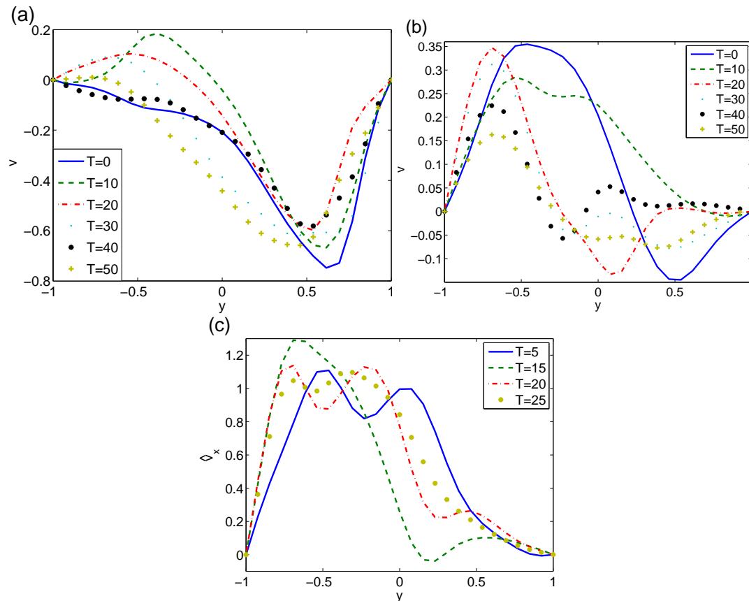
Figure 4. Velocity profile followed in time at a given spanwise position (that of Fig. 2) for different streamwise positions: (a): x = 45 , (b): x = 0 . (c): wall normal dependence of the growing Fourier mode, extracted from the DNS.
